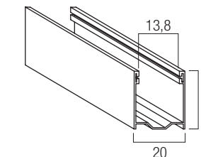
Guida in alluminio A25 GUAL..25M 20 x 25 mm
